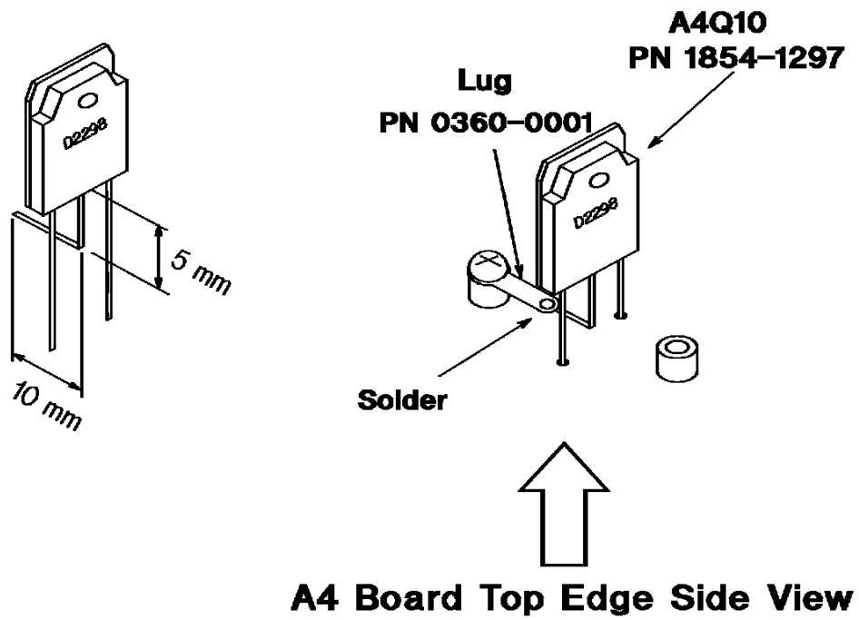
Fig.1 New Transistor Mounting
